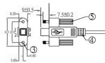
USB 2.0 B plug A110-507-001
